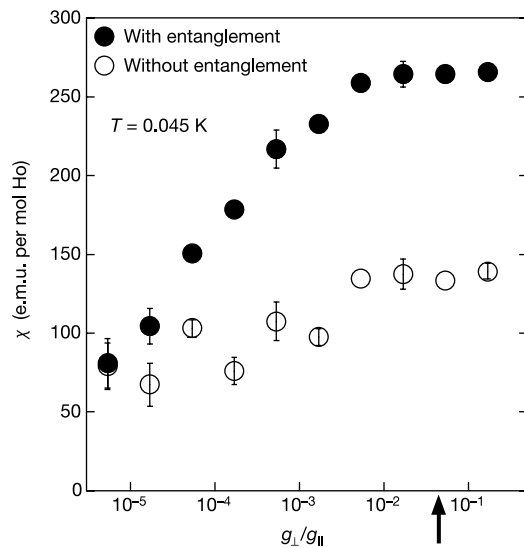
Figure 4 The change in susceptibility as the quantum entanglement is tuned by varying the ratio of the transverse and longitudinal magnetic g -factors, g_{\perp}/g_{\parallel} . An arrow denotes the value for \text{LiHo}_{0.045}\text{Y}_{0.955}\text{F}_4 . The full quantum susceptibility (filled circles) demonstrates extraordinary sensitivity to the slightest entanglement of the wavefunctions ( g_{\perp}/g_{\parallel} \approx 10^{-4} ), whereas the susceptibility calculated using the quantum energy levels but ignoring the entanglement (open circles) is relatively flat. Quantum entanglement produced by the off-diagonal terms, rather than spectral superposition, dominates the physics.
