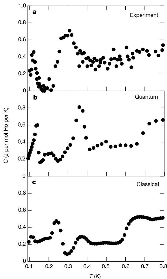
Figure 2 Comparison of the temperature-dependent experimental electronic specific heat C(T) for \text{LiHo}_{0.045}\text{Y}_{0.955}\text{F}_4 with different simulation techniques. a , Experimental data showing two sharp Schottky-like features dominating the thermal response. b , Quantum decimation, emphasizing how the well-defined energy levels result in a more complex temperature-dependent specific heat with greater resemblance to the experimental data, especially at low temperatures. Notably, there is the appearance of a sharp peak at 130 mK, close to a similar feature in the data. c , Classical decimation, demonstrating some success in calculating C(T) but with the characteristic sharp features occurring at incorrect temperatures. The features occur as k_B T moves through maxima in the distribution of dipolar couplings, and are affected as the concentration x varies; this distribution is granular, because the dipolar interaction is being sampled between points on a lattice rather than in continuous space.
