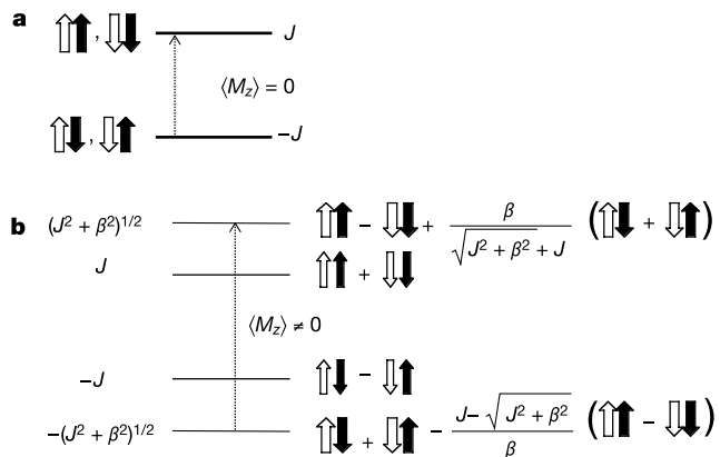
Figure 3 Diagram detailing the difference between the classical and the quantum decimation schemes. a , The classical energy levels calculated using equation (2). There are two doubly degenerate energy levels, designated +J and -J . Depending on the value of the angle formed by the Ising axis and the vector connecting the spins, the ground state -J can correspond to antiferromagnetic or ferromagnetic alignment of (i, j) . The eigenstates commute with \sigma_z , and there is no mixing between the ground-state doublet and the excited states. b , The quantum energy levels, showing the new entangled eigenstates. \beta is the off-diagonal term of the full dipolar interaction of equation (1), which reduces to the well-known hamiltonian of Ising spins in a transverse magnetic field in the limit of small (g_\perp/g_\parallel)^2 . The two doublets are split to produce eigenstates that are mixtures of the classical states. It is not only states from the same doublet that are mixed: \beta also yields a ground state that mixes ferromagnetic and antiferromagnetic classical states. Thus, the off-diagonal terms in the dipolar interaction introduce both a change in the spectrum (in the form of splittings of the doublets as well as shifts of the ‘ferromagnetic’ excited states relative to the ‘antiferromagnetic’ ground state), and mixing (or ‘entanglement’) of the classical states.
